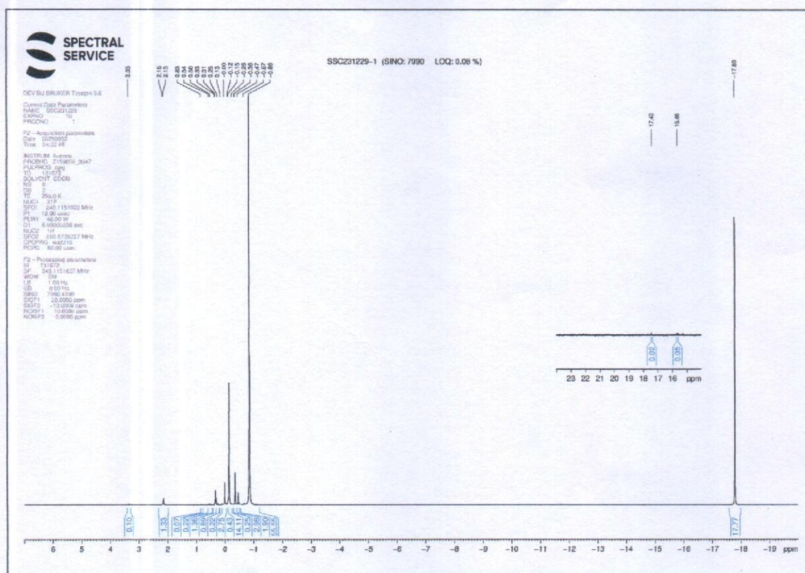
Fig. 1 ^{31}\text{P} -NMR spectrum of test item, Quantification (A)
